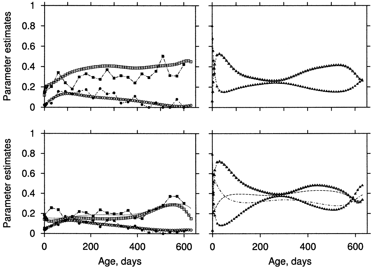
Figure 4. Random regression direct heritability estimates ( \square ), and animal ( \Delta ) and maternal ( \circ ) permanent environmental and residual ( \blacktriangle ) variance components as proportion of phenotypic variances. Univariate analysis direct heritability estimates ( \blacksquare ) and maternal permanent environmental variances ( \bullet ) as proportion of phenotypic variances. Data set 2 (bottom) and data set 3 (top). Animal permanent environmental (dash line) and residual (dot dash line) variances as proportion of phenotypic variances for data set 4 (bottom right).
