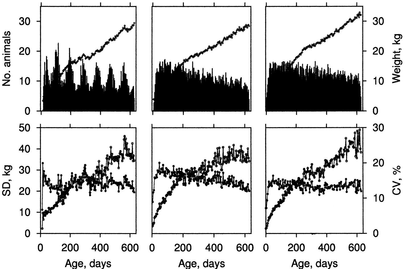
Figure 1. Top: weight means divided by 10 (+) and number of observations divided by 10 (bars). Bottom: standard deviations (○) and coefficient of variation (●), for data sets 1 (left), 2 (middle), and 3 (right), respectively.
